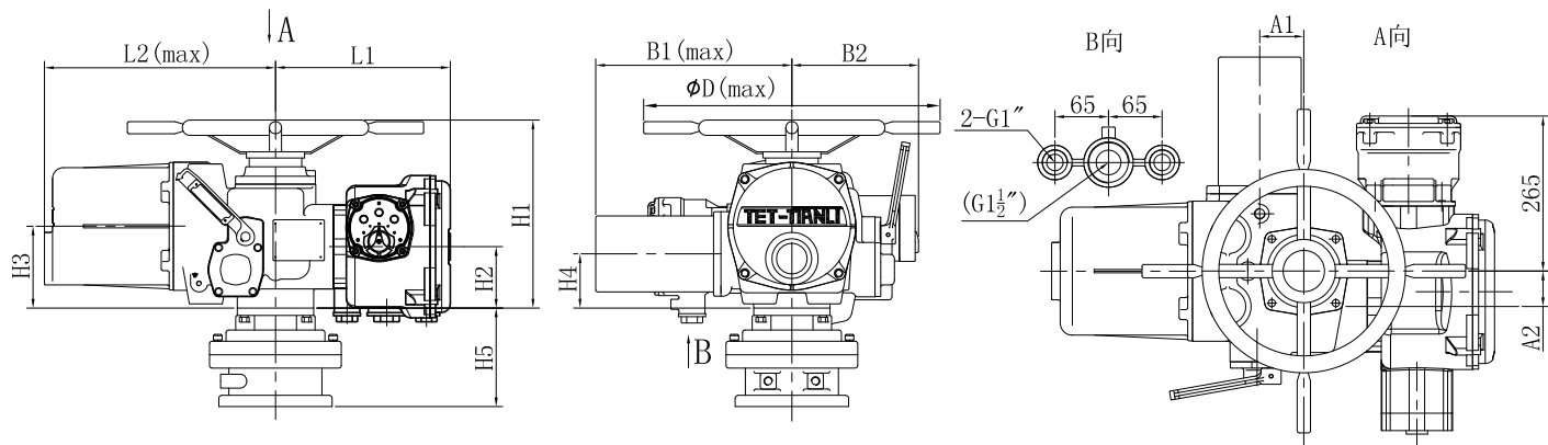
SMC-04~03Ex (IN) 带JA外形尺寸
